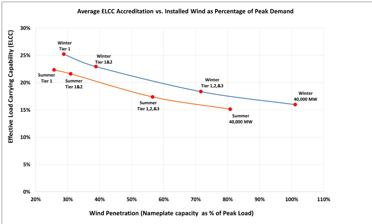
Figure 1. 2022 Average ELCC Accreditation
