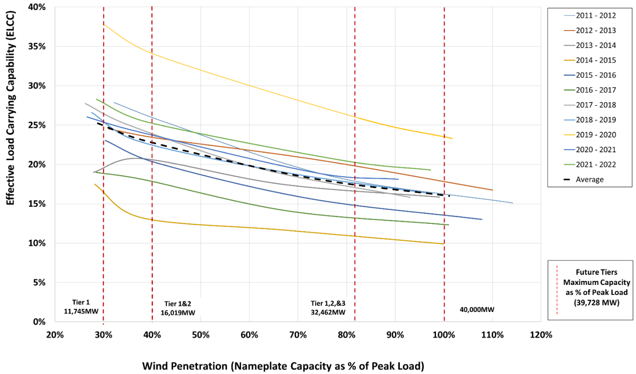
Figure 7: ELCC Winter Wind Results by Weather Year
